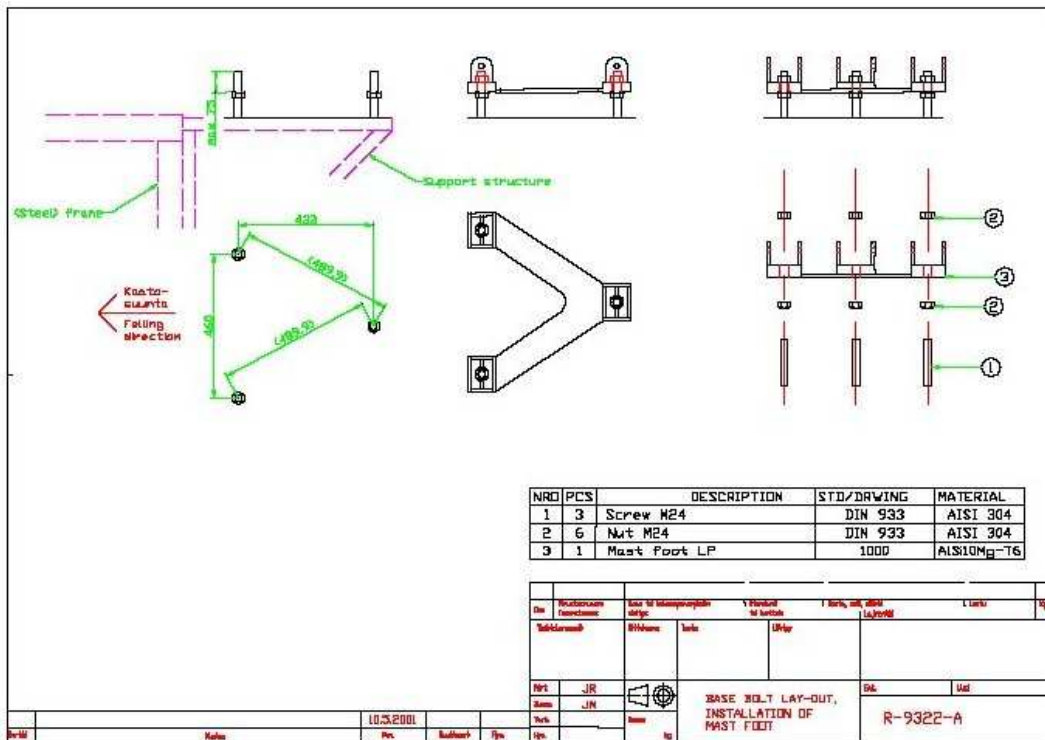
Base Plate Layout
