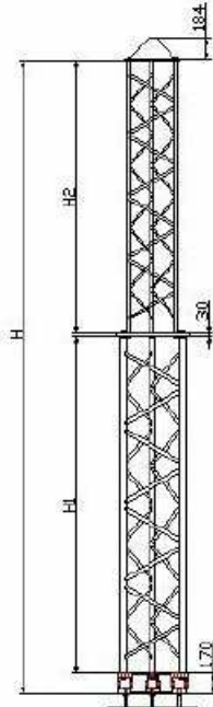
Cross Section 400 / 500 mm
